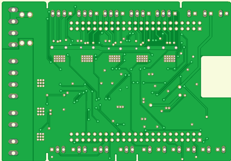
P018124 PCB view BOTTOM (bottomview)
