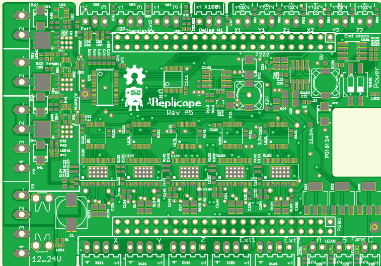
P018124 PCB view TOP (topview)
