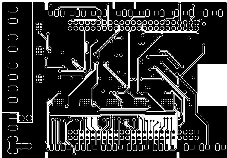
P018124 BOTTOM layer Image (topview)
