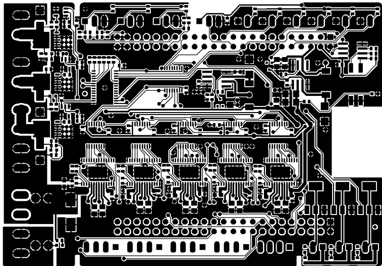
P018124 TOP layer Image (topview)
